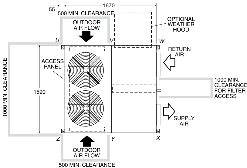
Fig. 1 OPA 430RKTBH – Horizontal Supply & Return Air
