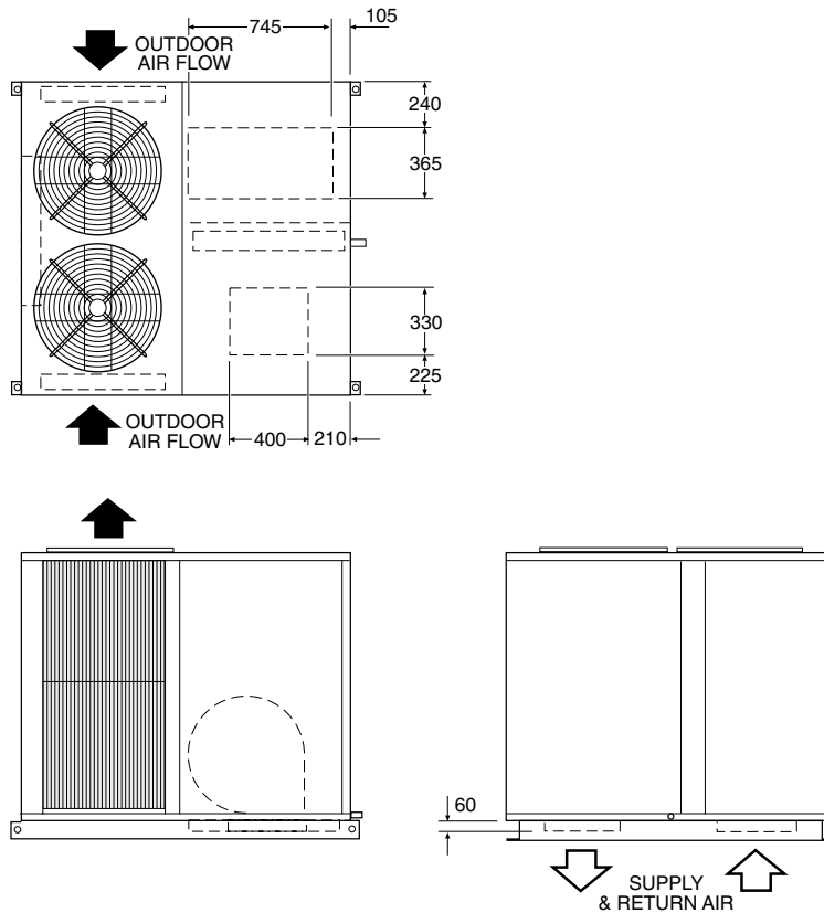
Fig. 2 OPA 430RKTBU – Downward Supply & Return Air
