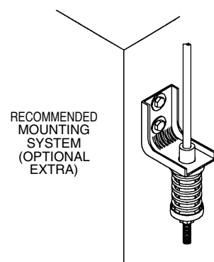
Fig. 2 Spring Mounting
