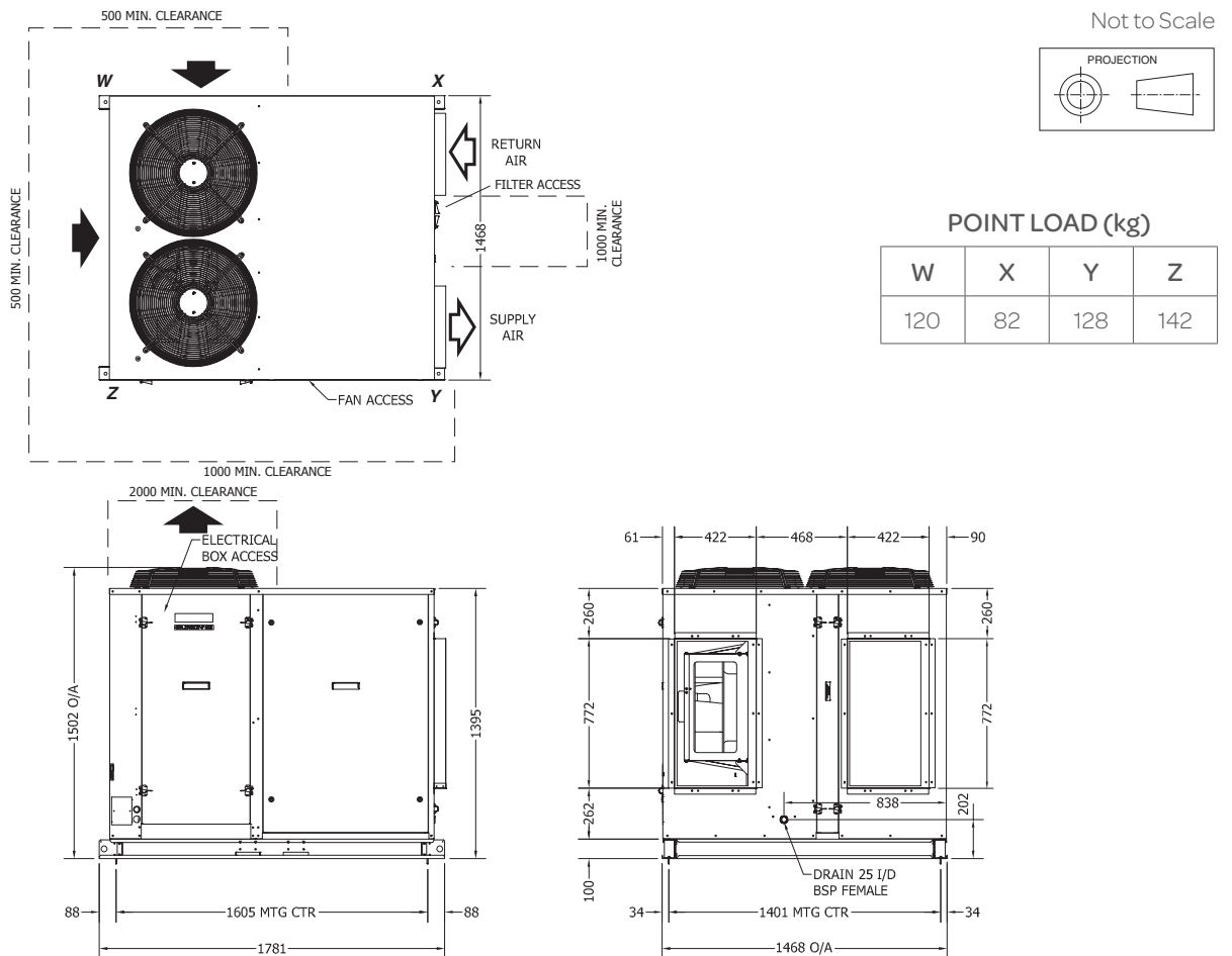
FIG. 1 OPA 336RKTFO1-P : HORIZONTAL SUPPLY & RETURN AIR
