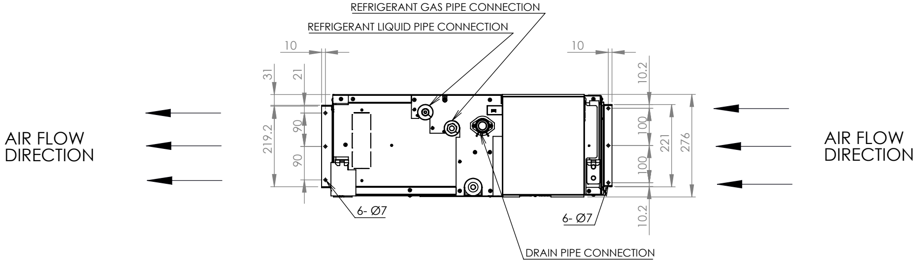
SIDE VIEW
