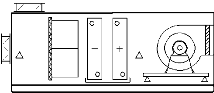
Standard DIDW
