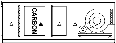
Carbon Filters
