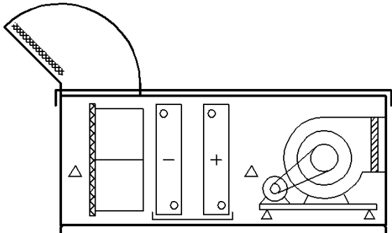
Carbon Filters
