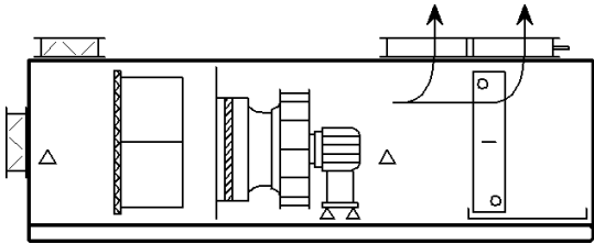
Multi-Zone
