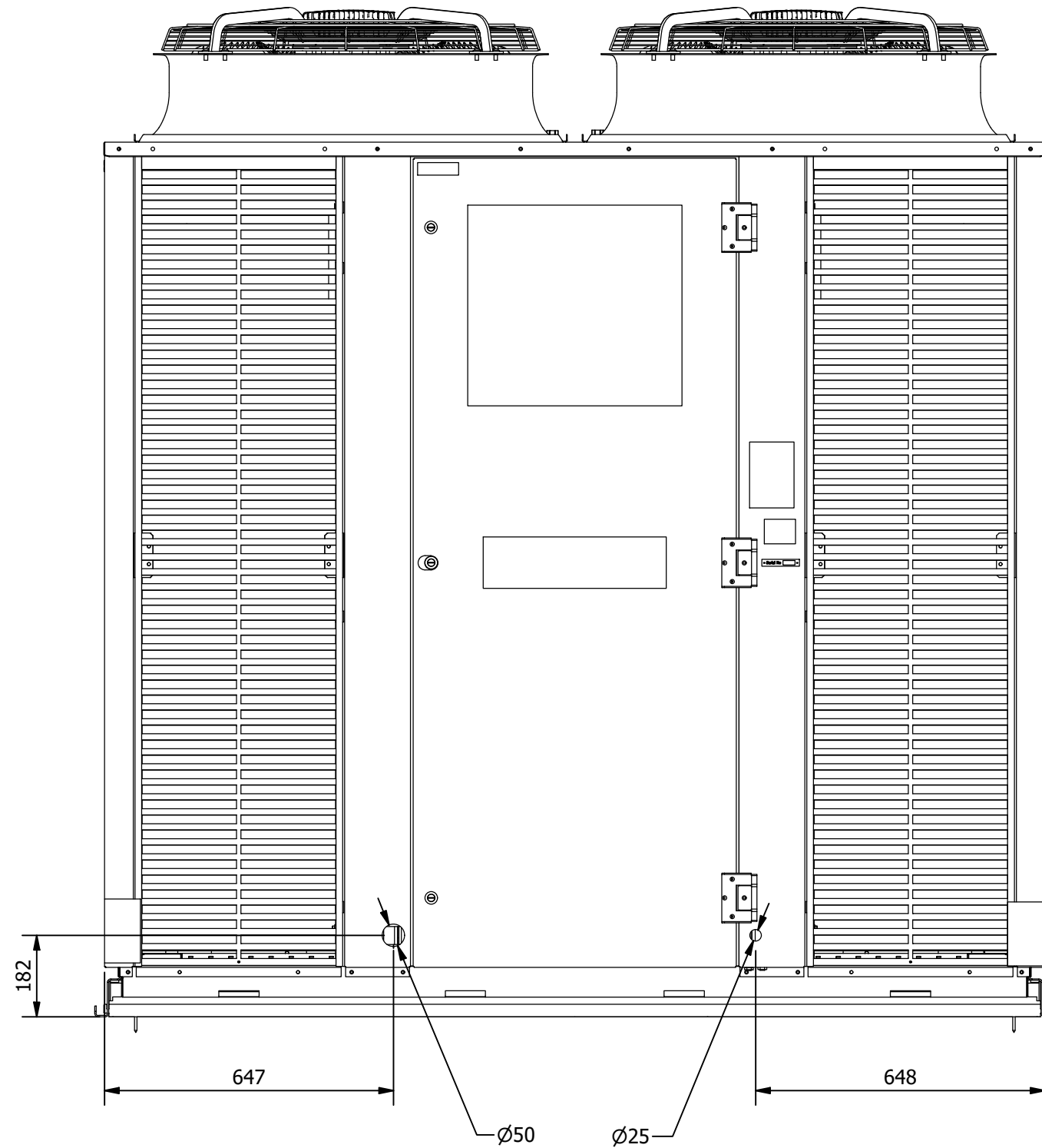
OPA 970 Cable Entrance Hole Dimensions
